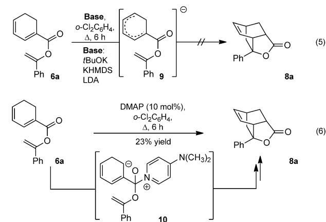
Scheme 1. Comparison between Brønsted base mediated and nucleophilic catalysis. DMAP = 4-dimethylaminopyridine, HMDs = hexamethyldisilazane, LDA = lithium diisopropylamide.
